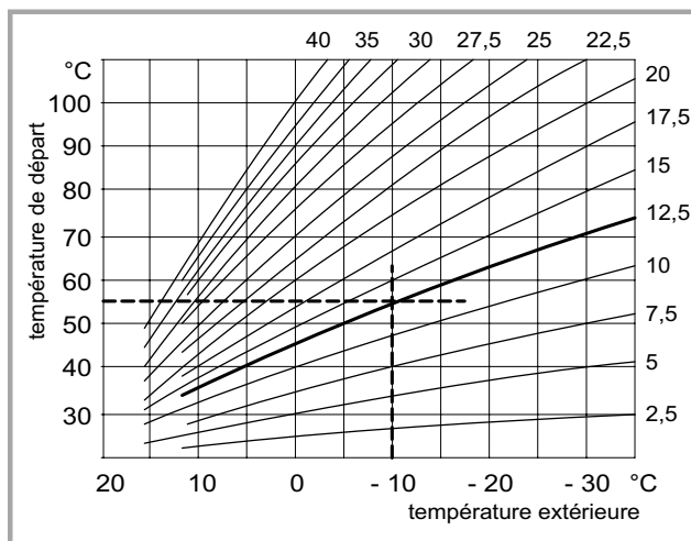
Figure 35 - Pente de chauffe
