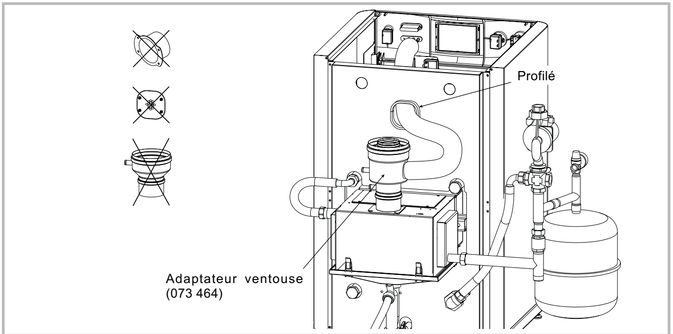
Figure 19 - Raccordement de la ventouse
